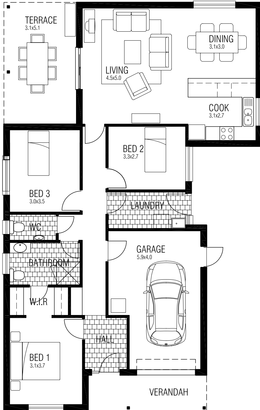
FLOOR PLAN
