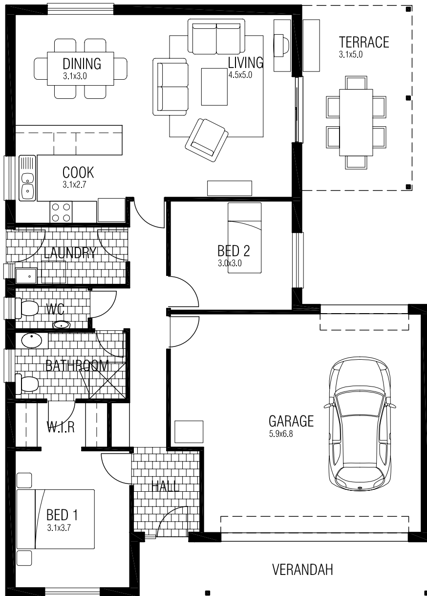
FLOOR PLAN
